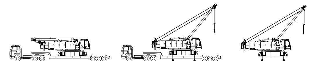
Step 1 Unloading
